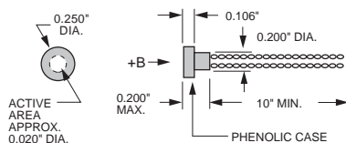
Axial Hall Sensors BHA-900, 910 & 921
